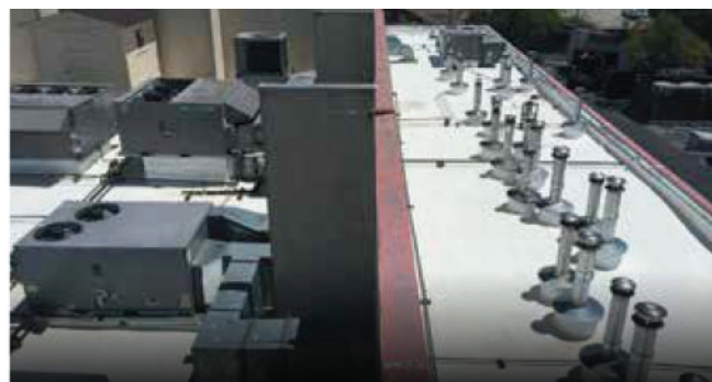
SPF provides self-flashing around all deck-mounted equipment and penetrations for this industrial manufacturing facility.
