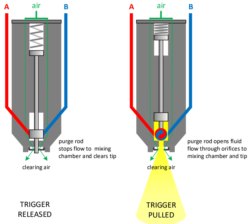
Figure 20 - Mechanical-purge gun schematic
