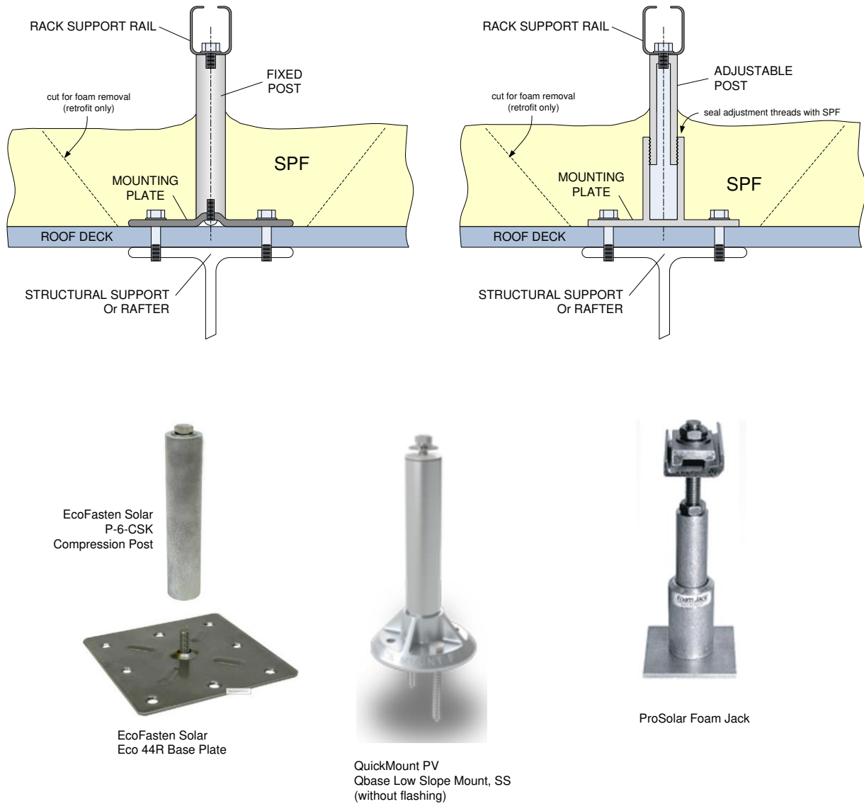
Figure 7 - Individual stand-offs
