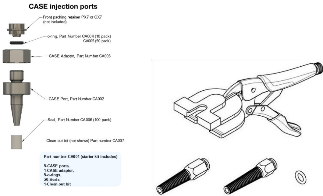
FIGURE 2 – Types of Injection Ports
